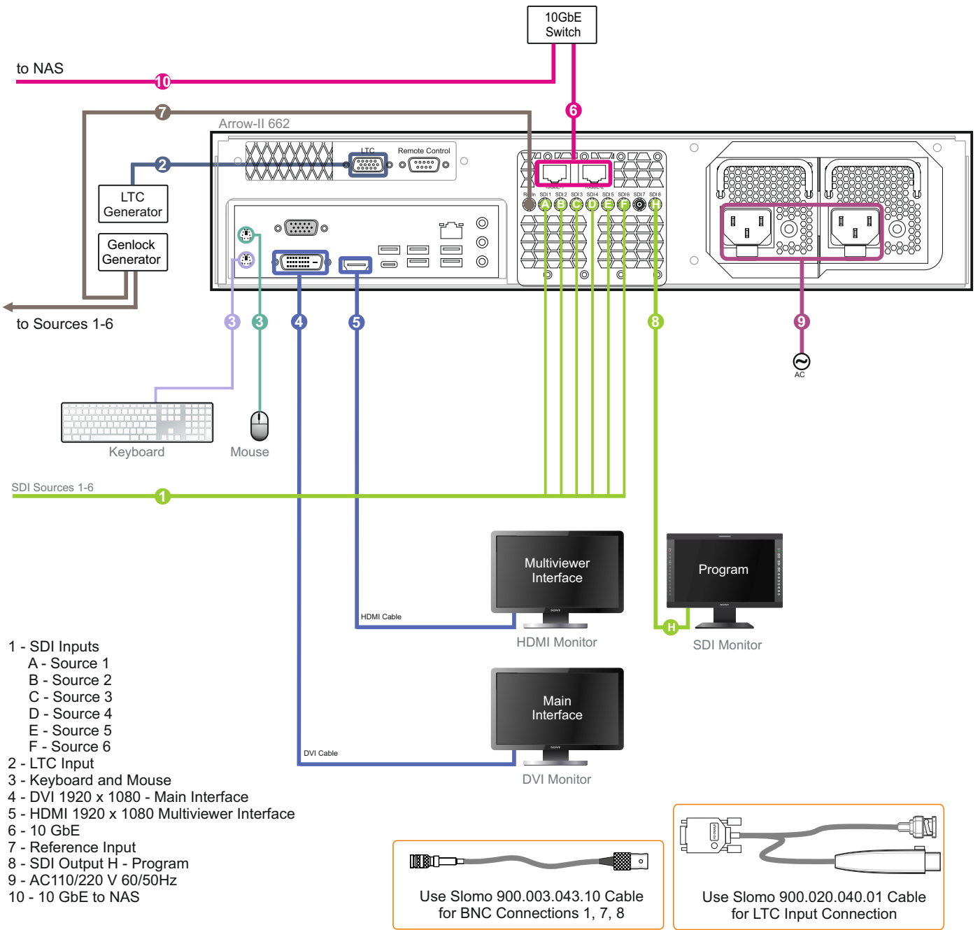
Connection diagram
