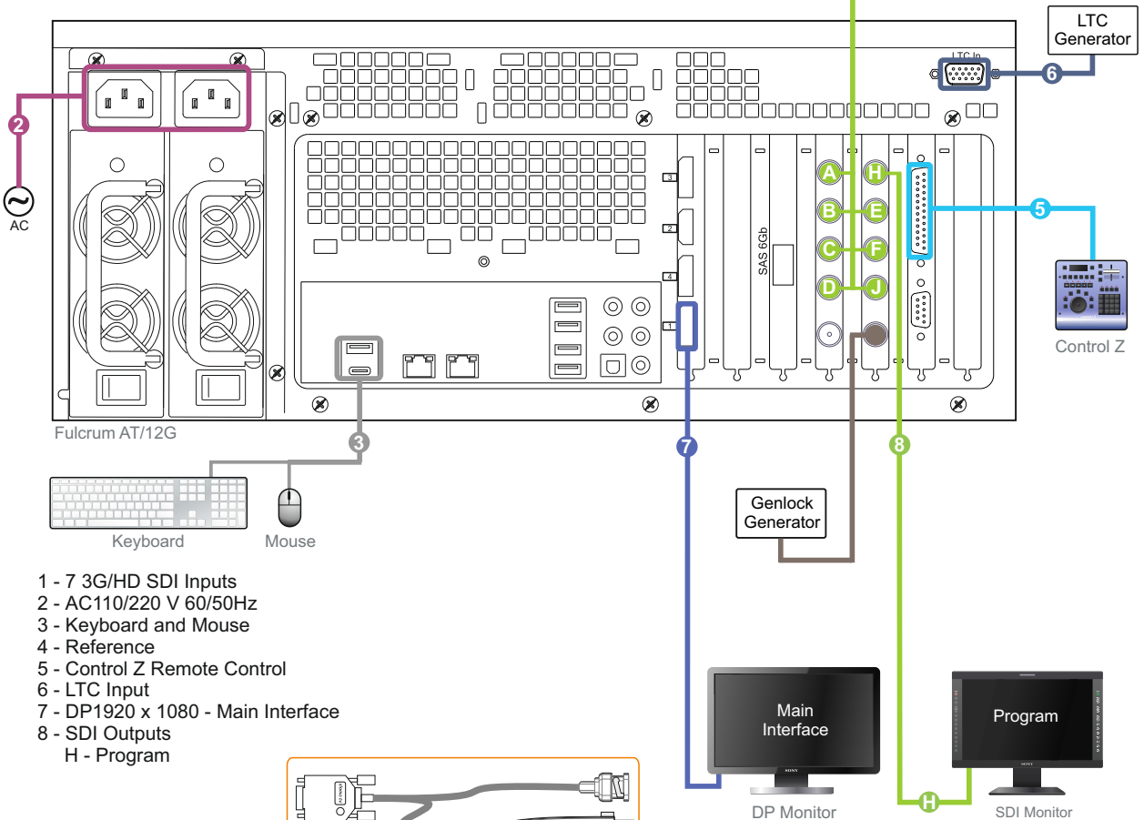
Use Slomo 900.020.040.01 Cable for LTC Input Connection
